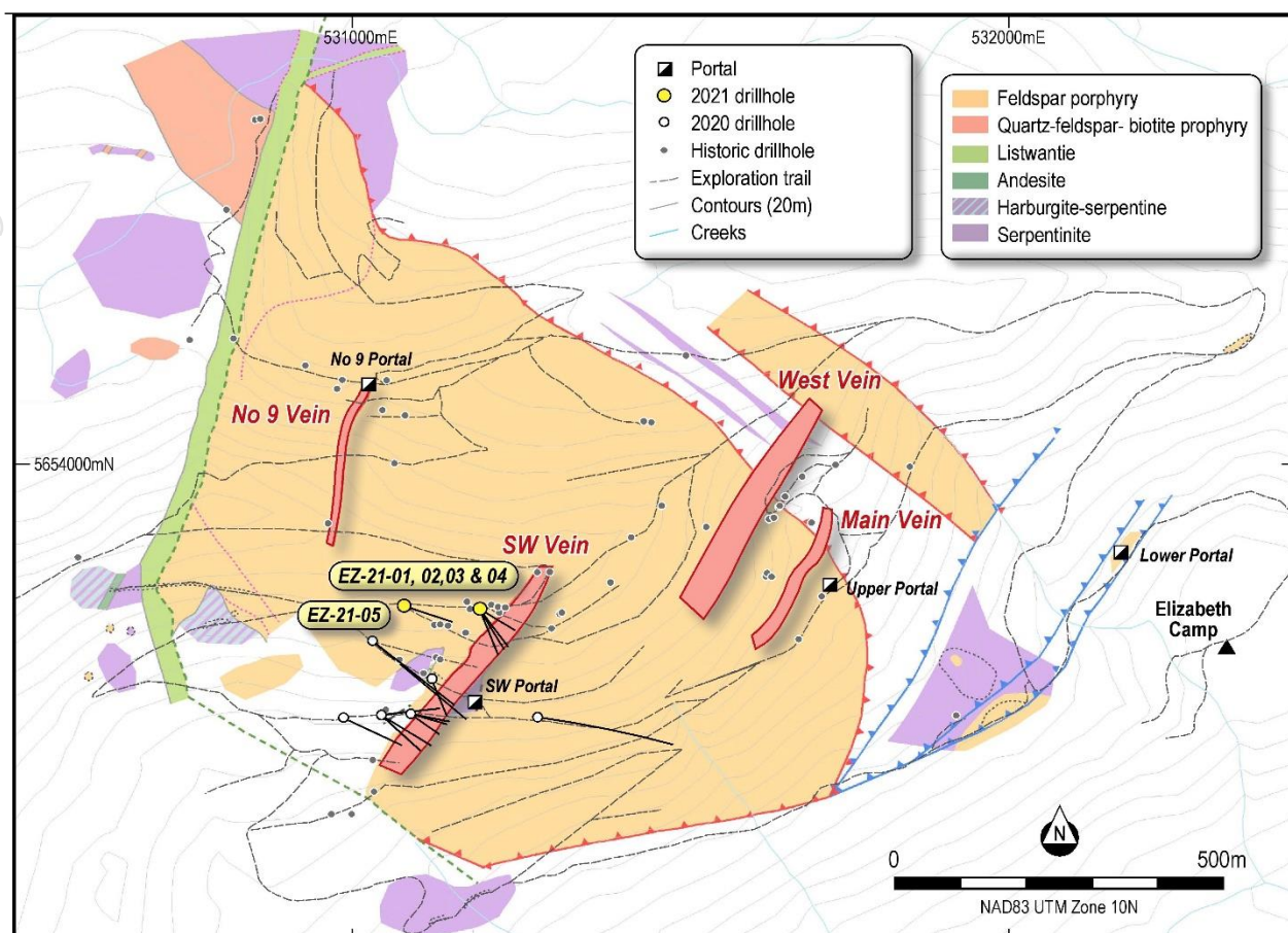
Figure 3 – Elizabeth Plan View Showing 2021 Drill Locations
