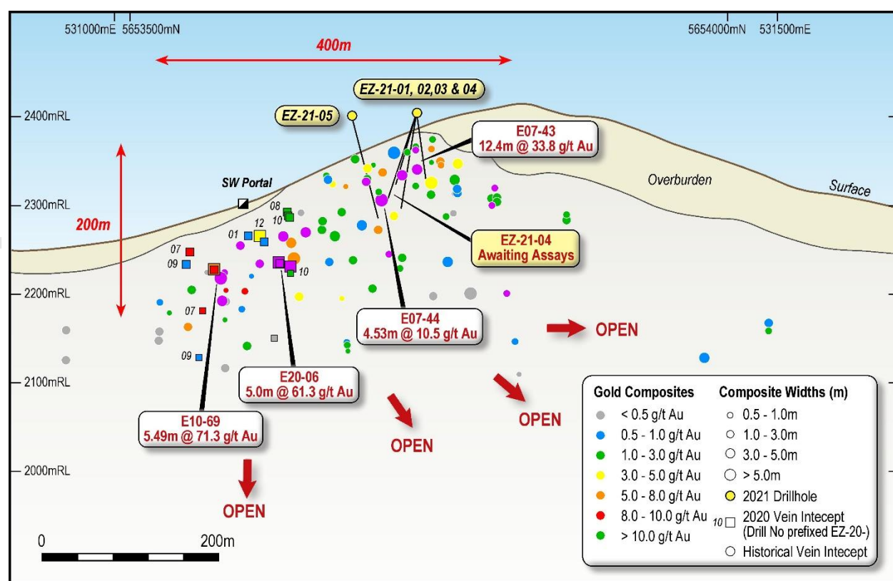
Figure 4 – Elizabeth SW Vein Long Section (looking Northwest)
